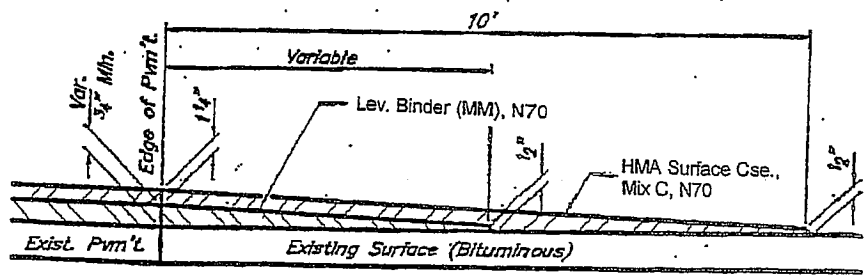
SECTION A-A PRIVATE ENTRANCE
