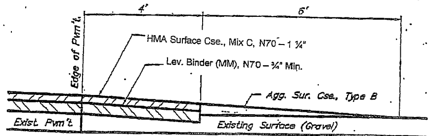
SECTION A-A PRIVATE ENTRANCE - GRAVEL
