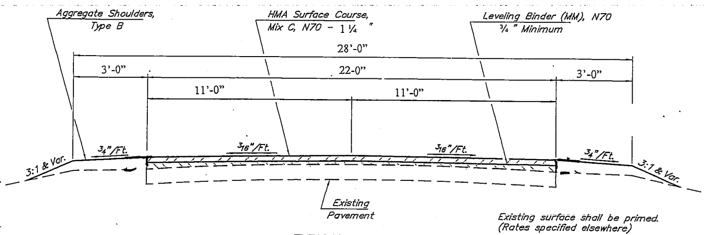
TYPICAL SECTION
