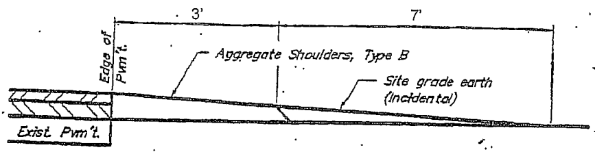
SECTION A-A FIELD ENTRANCE
