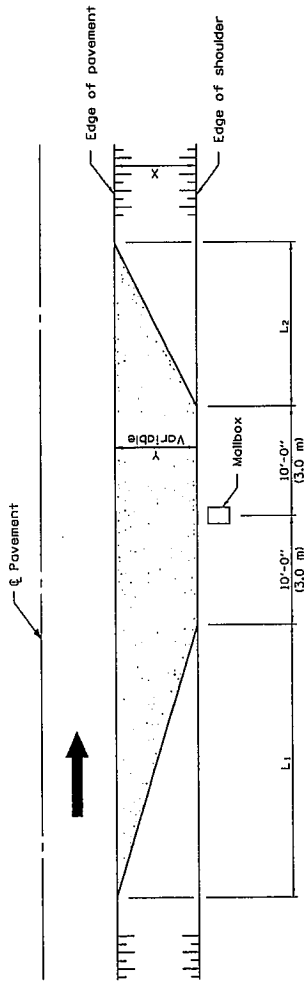
TYPICAL APPLICATION
