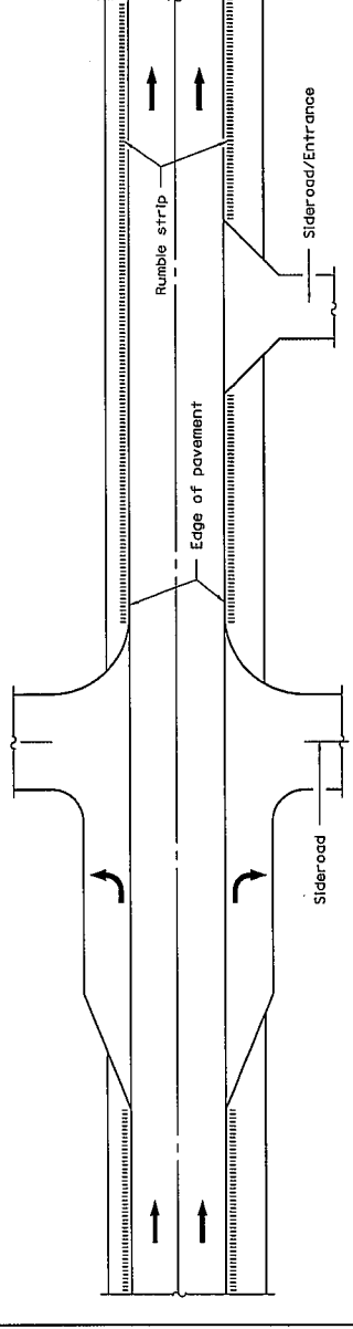
HALF PLAN
