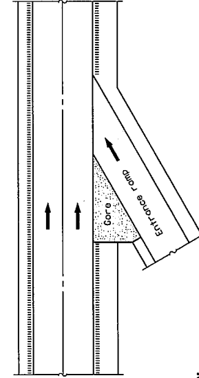
HALF PLAN
