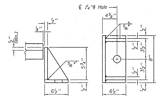
SIDE RETAINER
