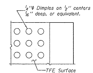
PLAN-TFE SURFACE
