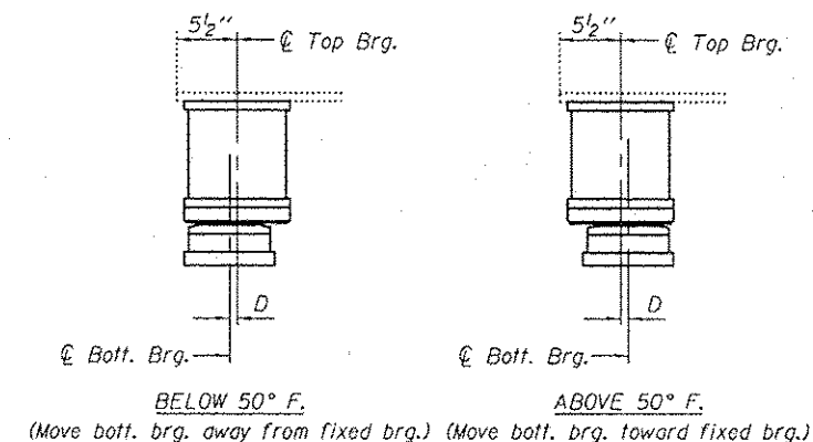
SETTING ANCHOR BOLTS AT EXP. BRG. D = 1/8" per each 100' of expansion for every 15° temp. change from the normal temp. of 50°F.
