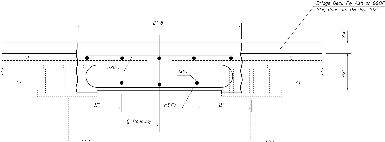
SECTION F-F
