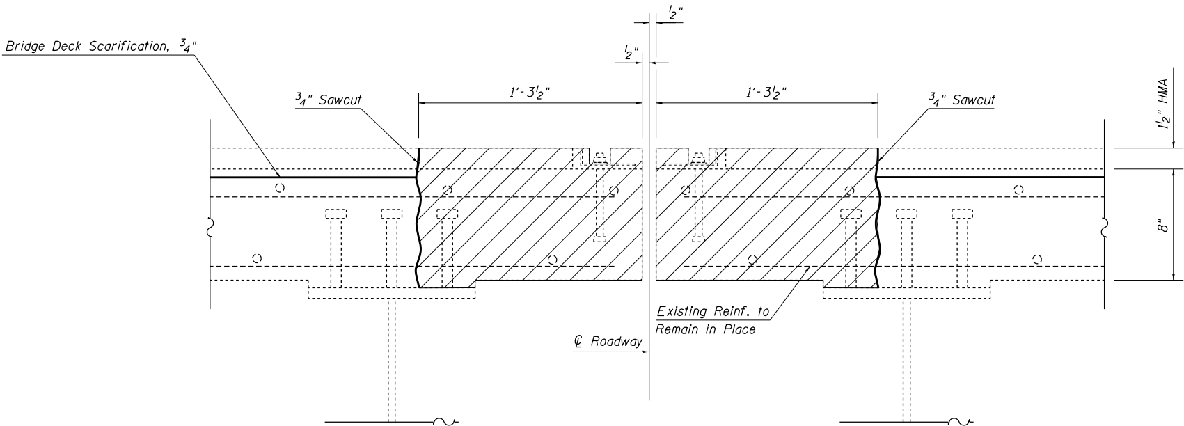
SECTION E-E
