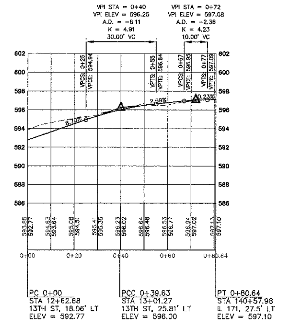
NW PROFILE
