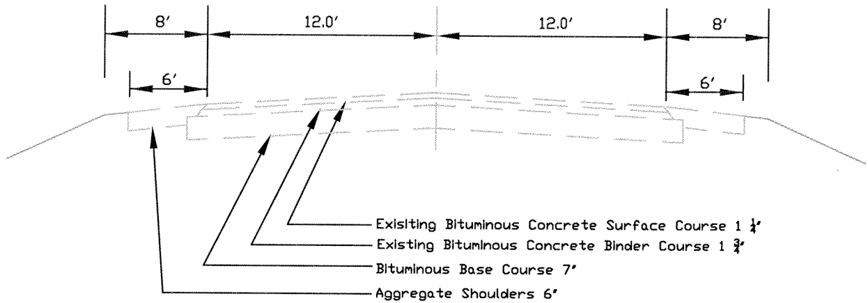
EXISTING TYPICAL SECTION Original Construction Section: 89-00164-01-FP STA. 26+67.30 TO STA. 40+03.30 STA. 40+97.30 TO STA. 108+35.10 STA. 110+40.60 TO STA. 152+31.00
