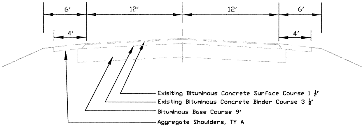
EXISTING TYPICAL SECTION Original Construction Section: 06-00090-07-WR STA. 9+70.00 TO STA. 39+06.60
