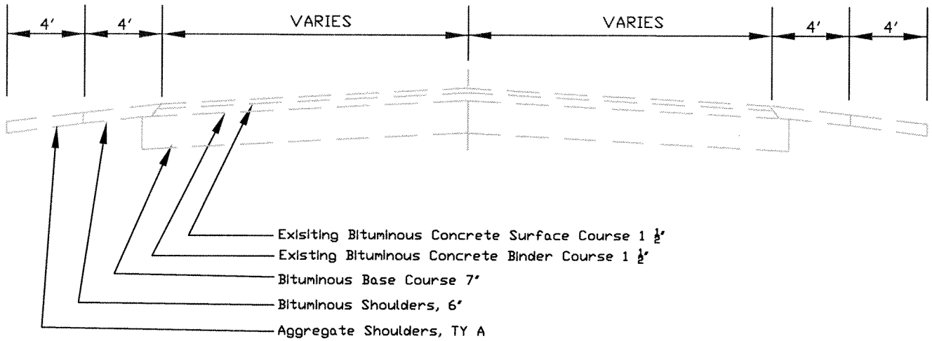
EXISTING TYPICAL SECTION Original Construction Section: 99-00090-03-TL STA. 152+31.00 TO STA. 156+07.00
