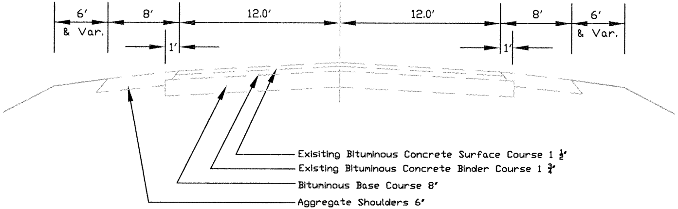
EXISTING TYPICAL SECTION Original Construction Section: 88-00051-01-FP STA. 56+50.00 TO STA. 85+51.83 STA. 87+34.31 TO STA. 133+35.00
