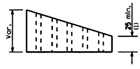
PARAPET WOOD BLOCK-OUT DETAIL
