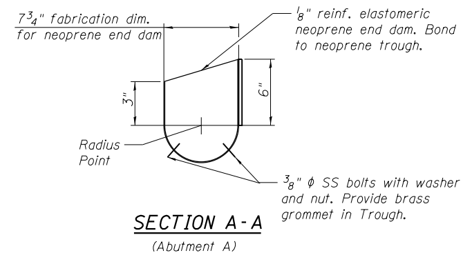
SECTION AT END OF TROUGH
