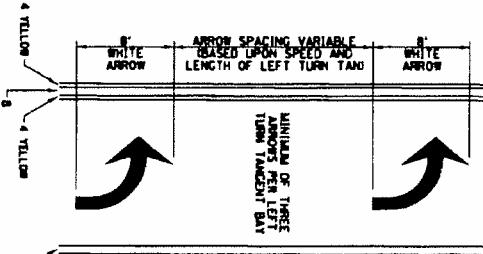
ARROW LAYOUT
