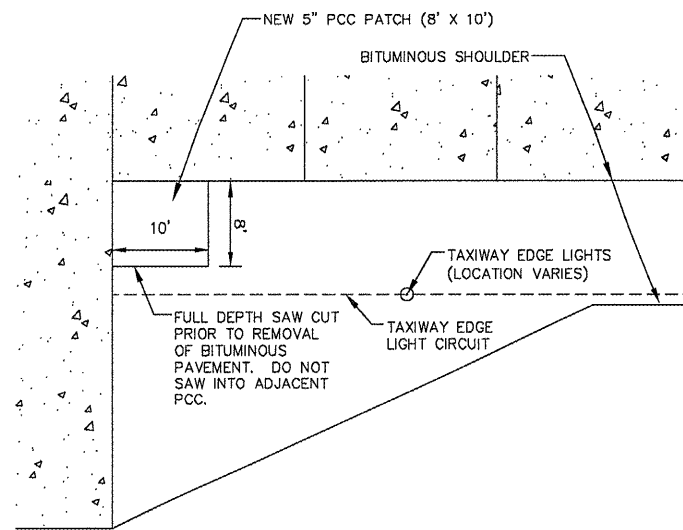
SHOULDER REPAIR — PLAN VIEW NOT TO SCALE
