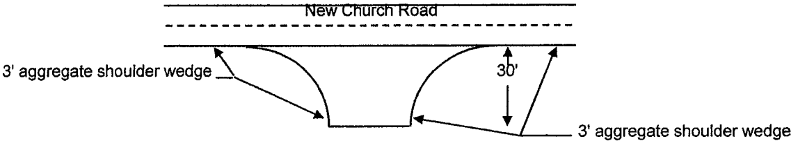
DETAIL OF SIDEROAD
