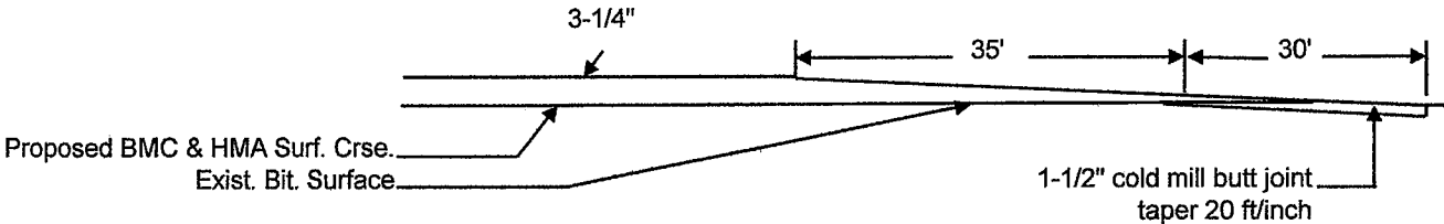
DETAIL OF END TAPERS
