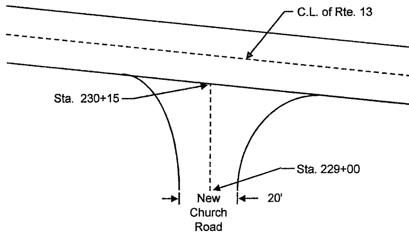
DETAIL OF INTERSECTION WITH RTE. 13
