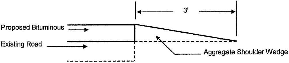
DETAIL FOR AGGREGATE SHOULDER WEDGE
