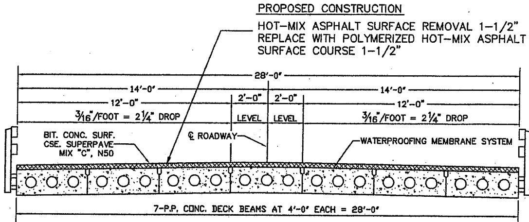
CROSS SECTION S.N. 014-3014
