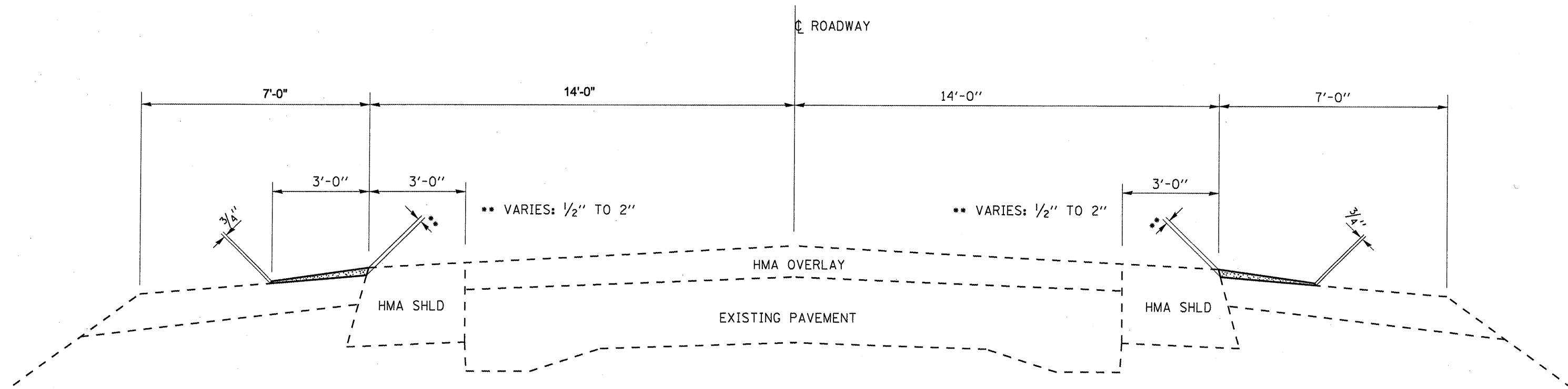
TYPICAL SECTION FAS ROUTE 332 (IL 1)
