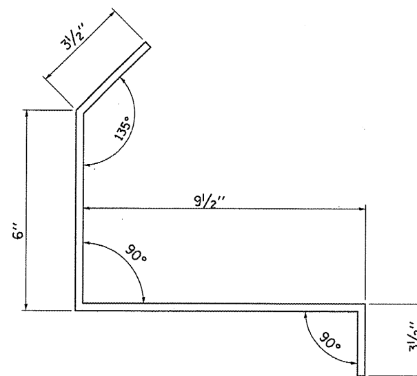
1/4" x 2" x 1'-10 1/2" BRACKET (2 REQUIRED PER BEAM)
