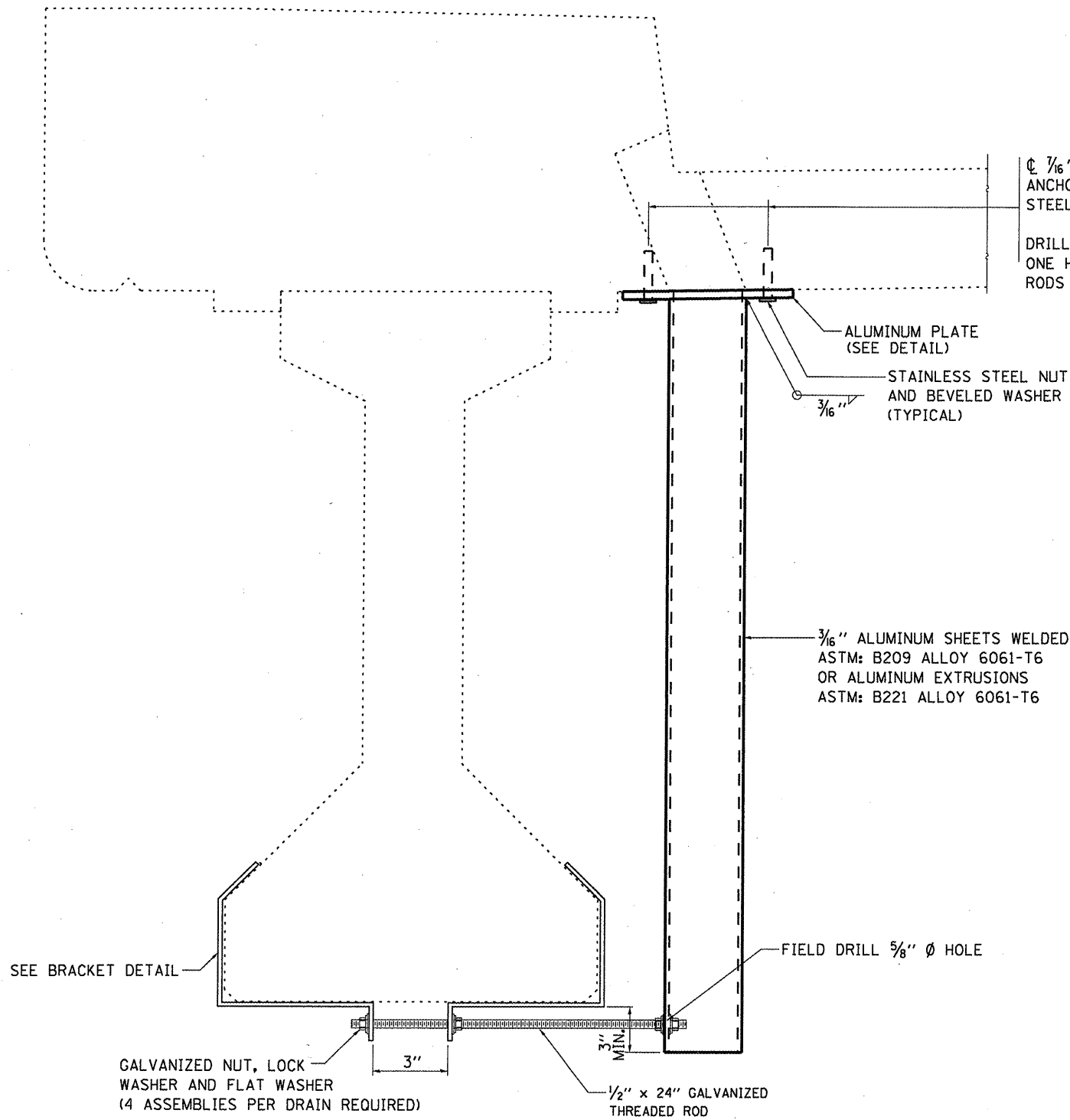
CURB ELEVATION
