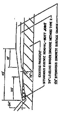
TYPICAL TAPER
