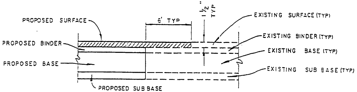
SECTION B-B
