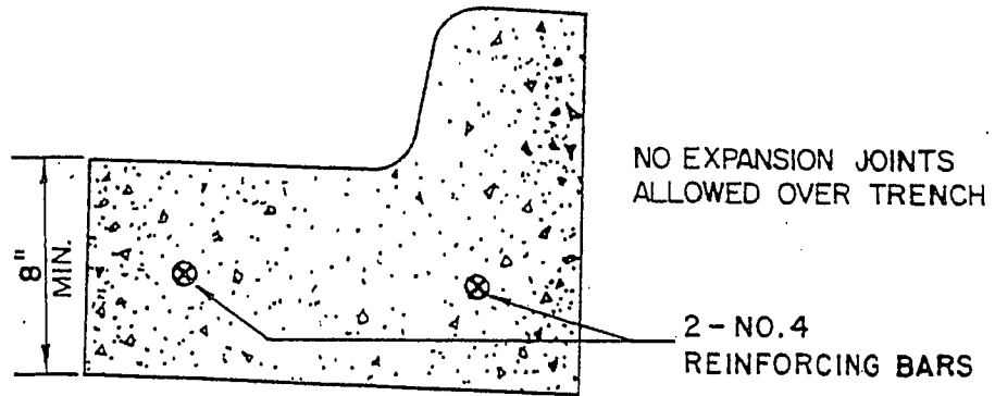
TYPICAL PLACEMENT IN CURB & GUTTER SECTION
