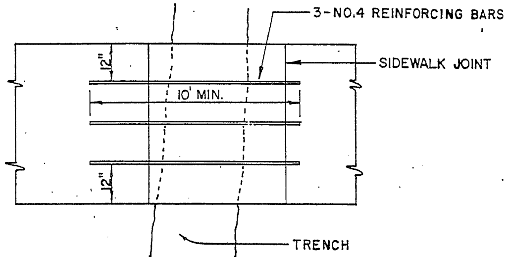
TYPICAL PLACEMENT IN SIDEWALK SECTION
