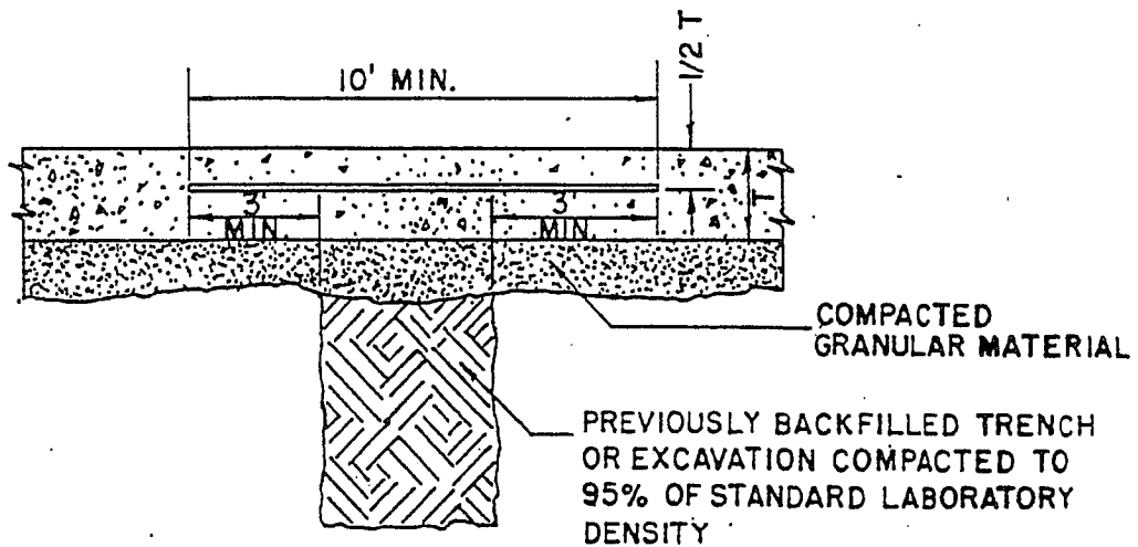
TYPICAL BAR LENGTH REQUIREMENTS OVER TRENCH
