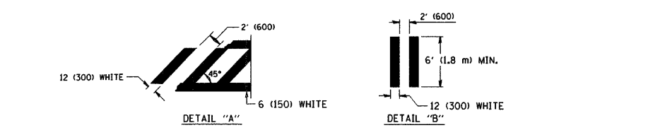
TYPICAL CROSSWALK MARKING
