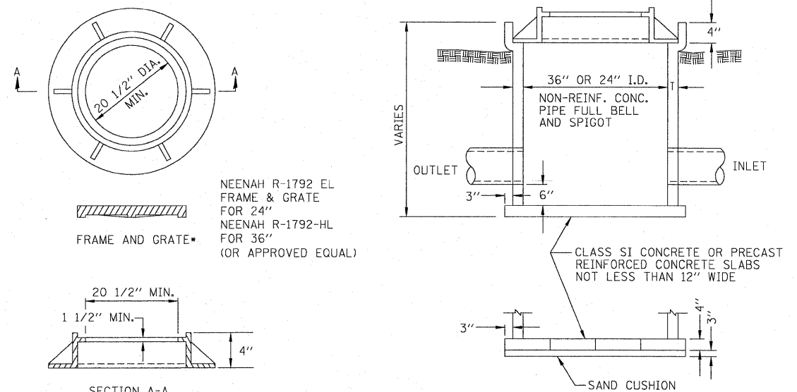
FIELD TILE JUNCTION VAULT DETAILS
