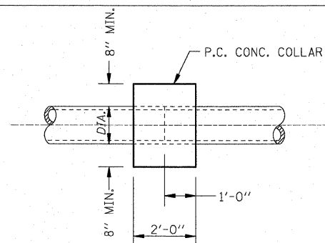
CONCRETE COLLAR DETAIL
