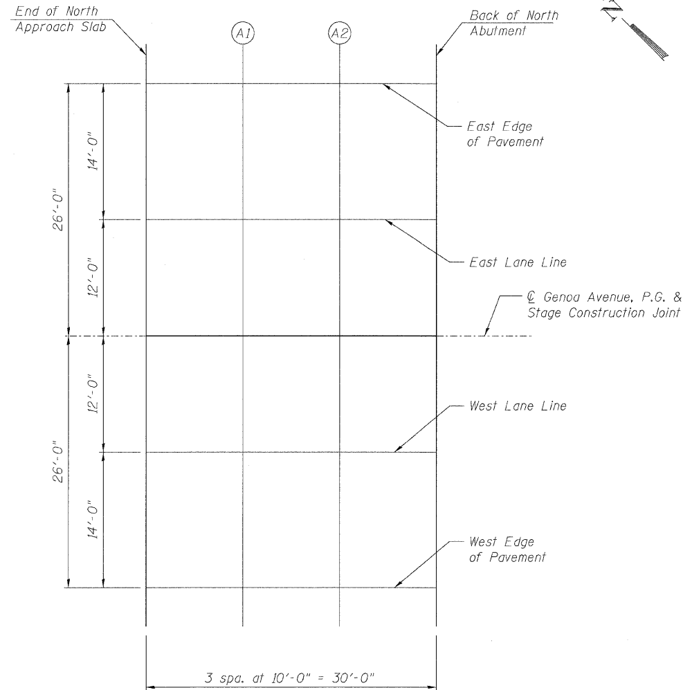
PLAN
