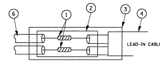
PRE-FORMED LOOP DETAIL "B" LOOP-TO-CONTROLLER SPLICE
