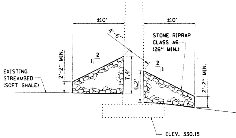
PIER 2 LOOKING NORTH DIMENSIONS PARALLEL TO TRAFFIC
