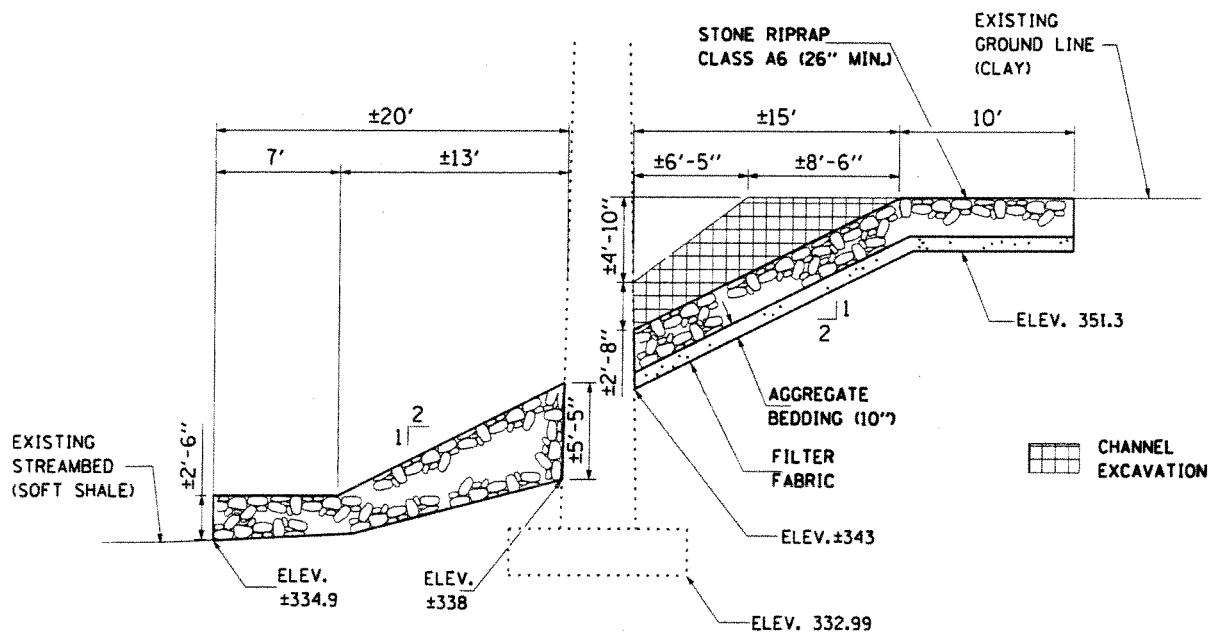
PIER 3 LOOKING NORTH DIMENSIONS PARALLEL TO TRAFFIC
