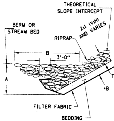
TOE DETAIL (A)
