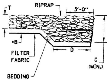
FLANK OR TOE DETAIL (B)
