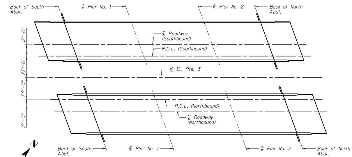
DECK LAYOUT
