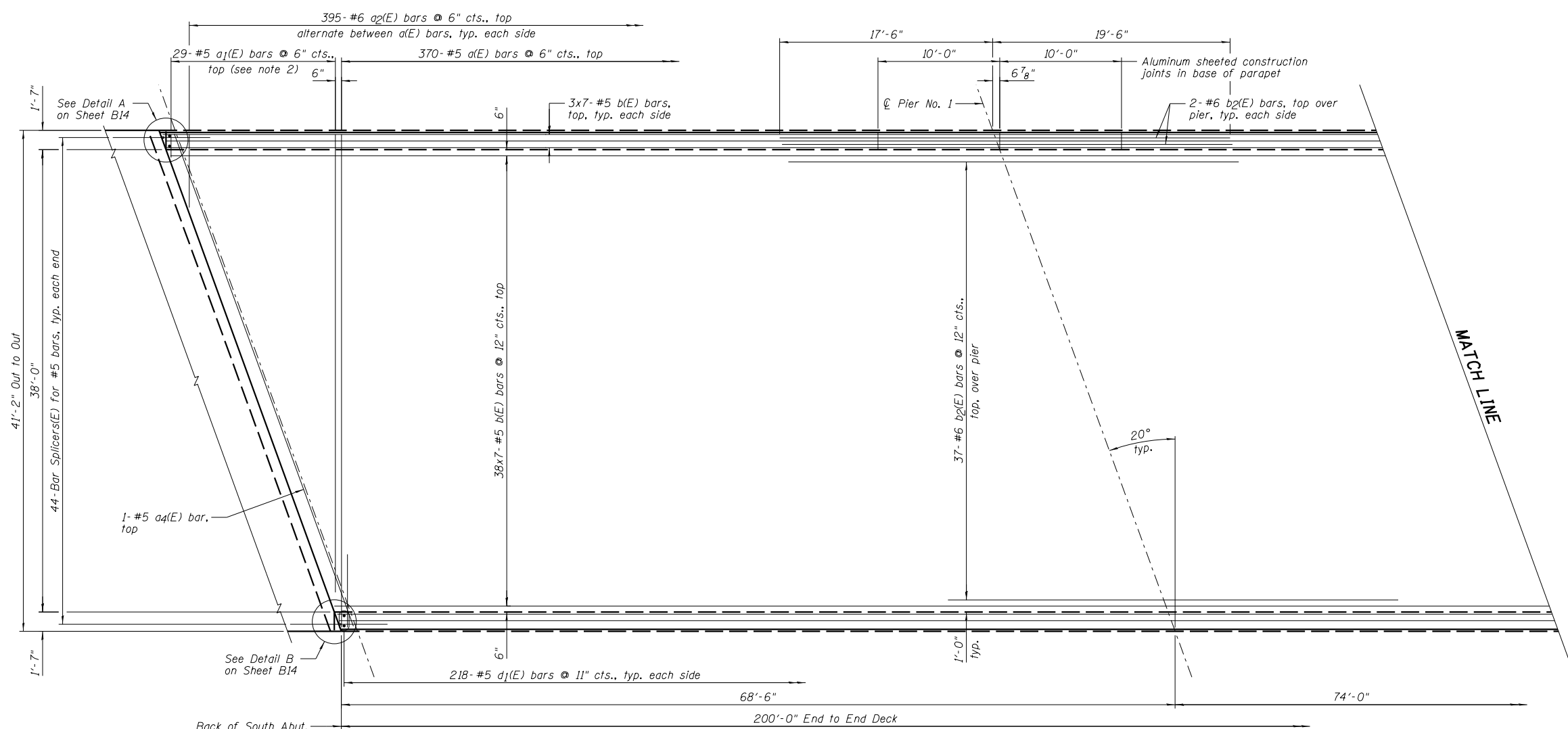
HALF PLAN
