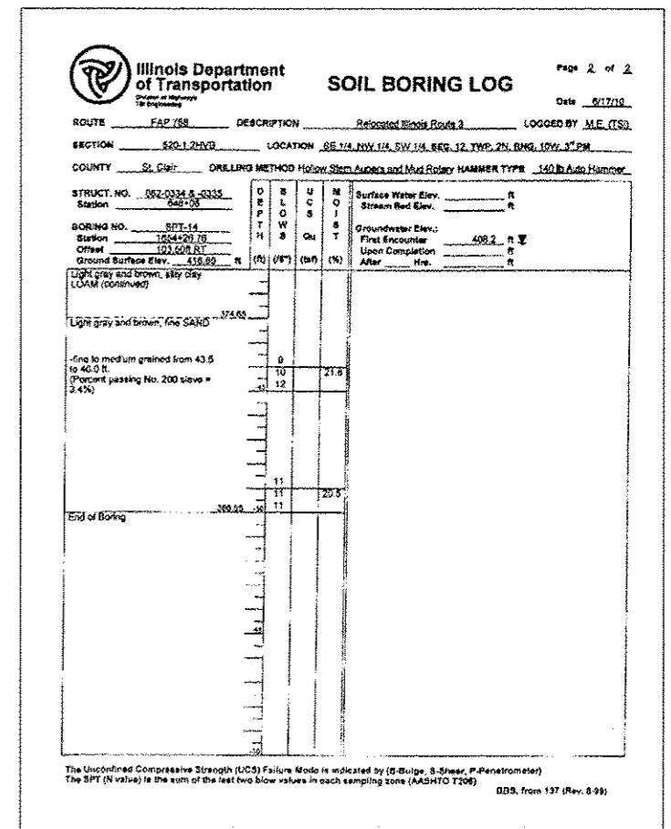
BORING SPT-14 (2 of 2)
