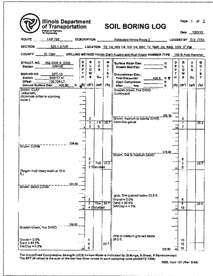
BORING SPT-13 (1 of 2)
