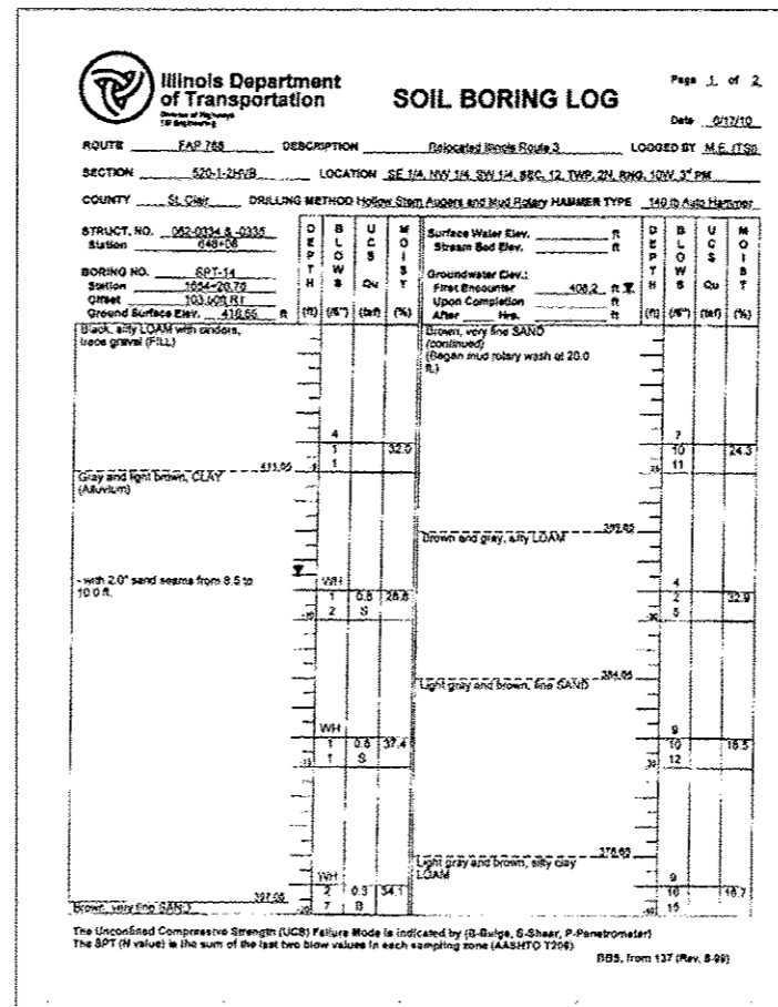
BORING SPT-14 (1 of 2)
