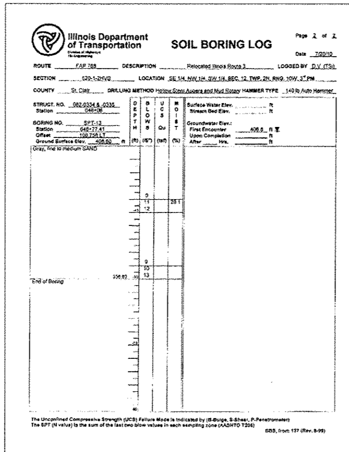
BORING SPT-13 (2 of 2)
