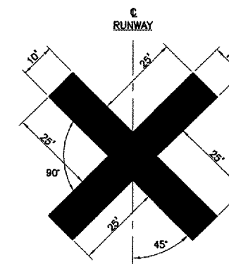
CLOSED RUNWAY MARKING DETAIL
