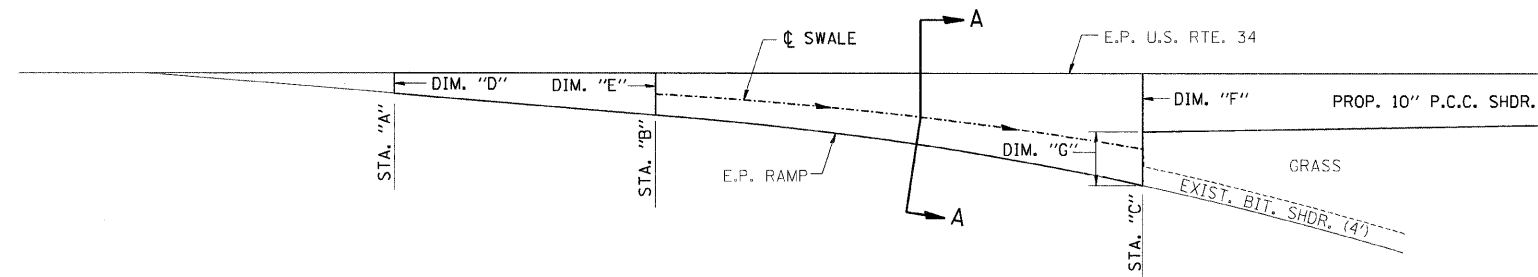
PLAN VIEW
