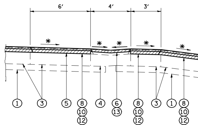
SECTION A-A (RAMP C)
