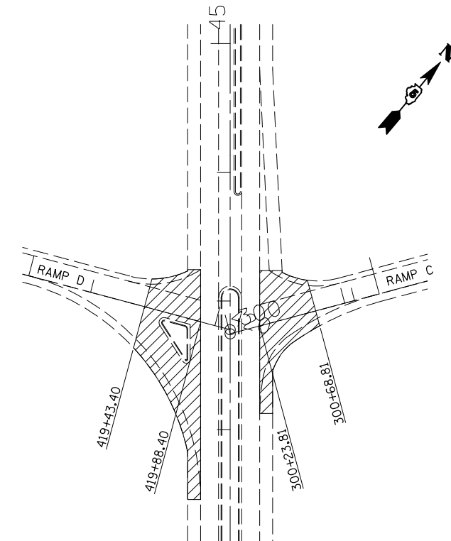
INTERSECTION OF FAP 135 WITH RAMP C & RAMP D
