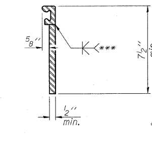
WELDED RAIL
