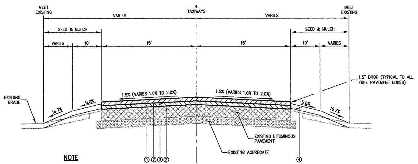
TYPICAL TAXIWAY OVERLAY SECTION
