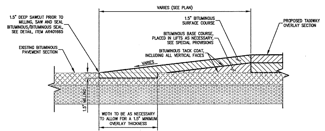
BITUMINOUS TAPER DETAIL
