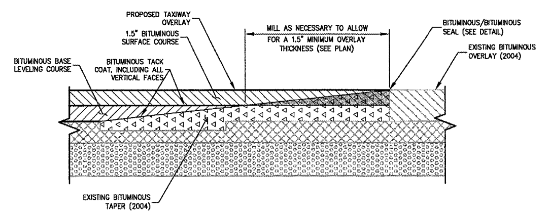
BITUMINOUS MILLING DETAIL (WHEN MEETING 2004 OVERLAY) (SEE PLAN FOR LOCATIONS)
