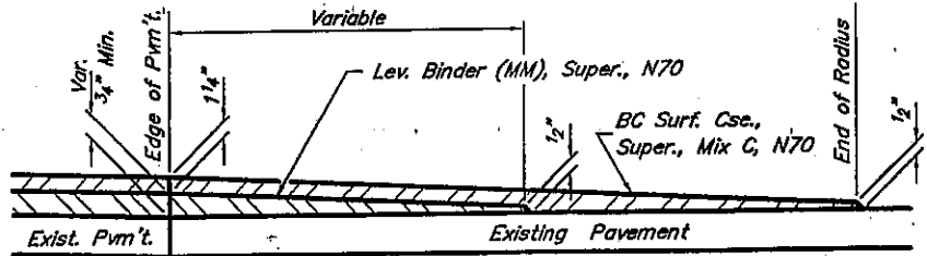
SECTION A-A SIDE ROAD (Est. No. = 12)
