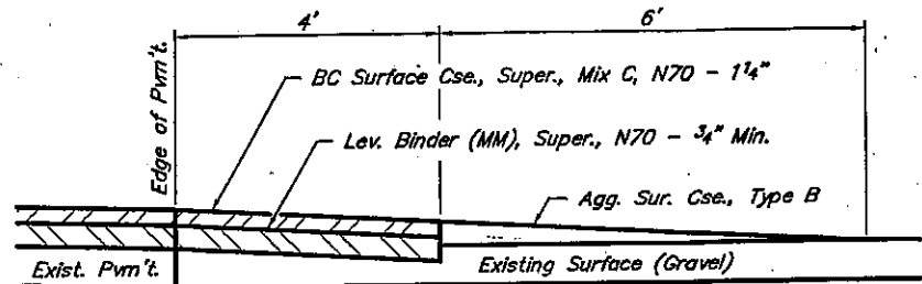
SECTION A-A PRIVATE ENTRANCE - GRAVEL (Est. No. = 103)
