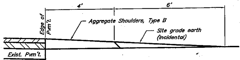
SECTION A-A FIELD ENTRANCE (Est. No. = 21)
