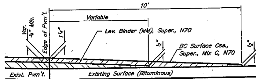
SECTION A-A PRIVATE ENTRANCE - BITUMINOUS (Est. No. = 10)
