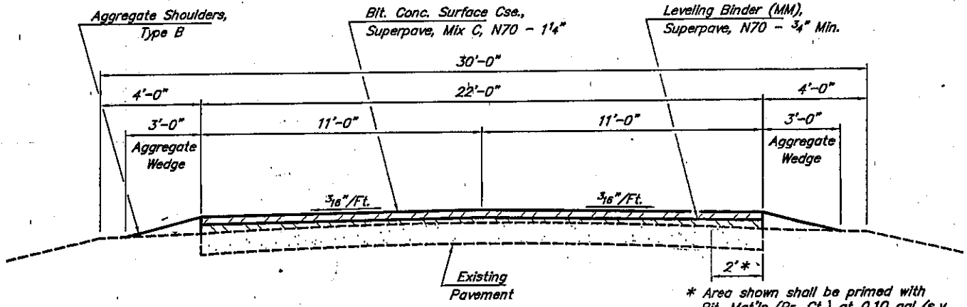
TYPICAL SECTION
