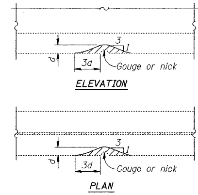
GRINDING DETAIL REPAIR 15 & 16
