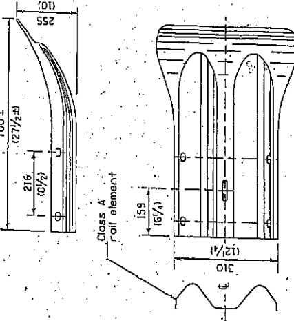
END SECTION
