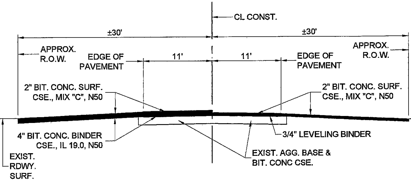
AT TYPICAL CROSS SECTION #1
