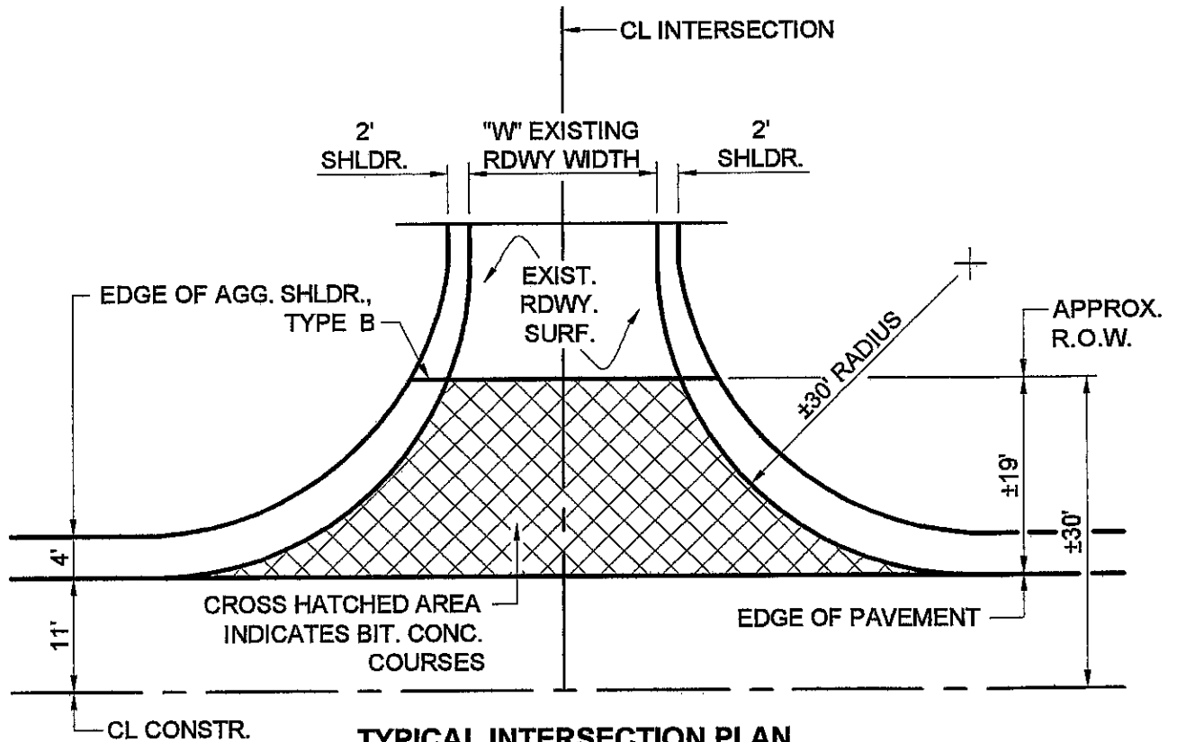
TYPICAL INTERSECTION PLAN
