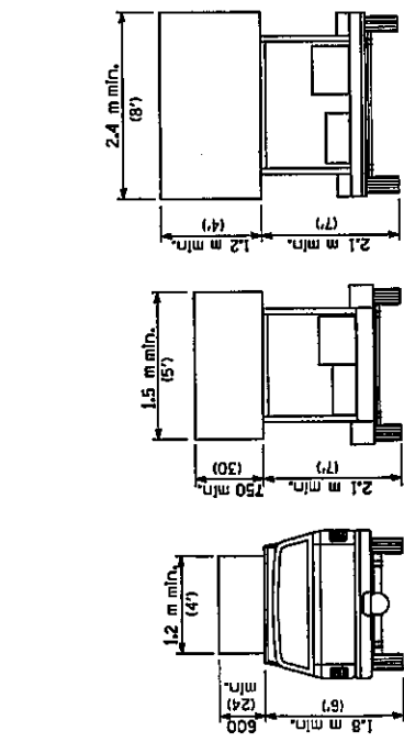
TYPE B ROOF OR TRAILER MOUNTED
