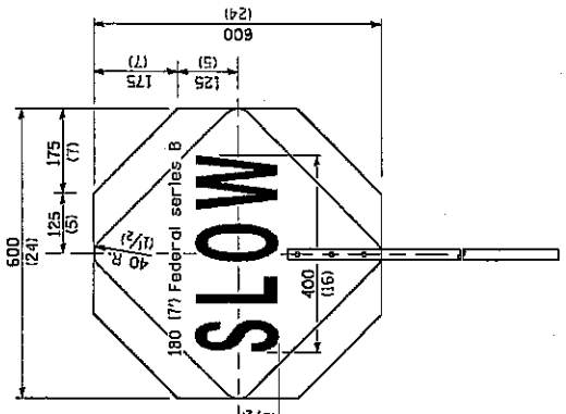
REVERSE SIDE
