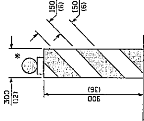
VERTICAL BARRICADE
