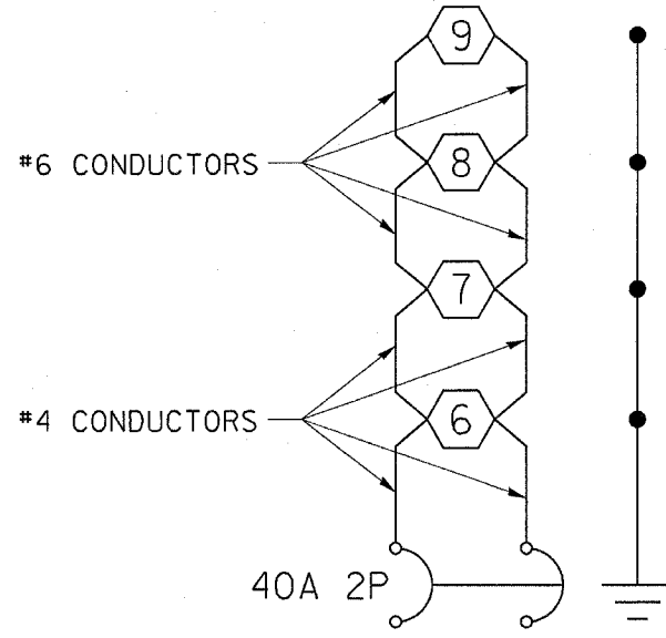
CIRCUIT 2
