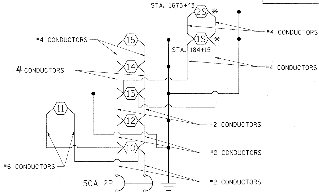
CIRCUIT 4
