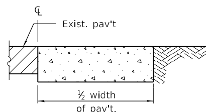
SECTION C-C
