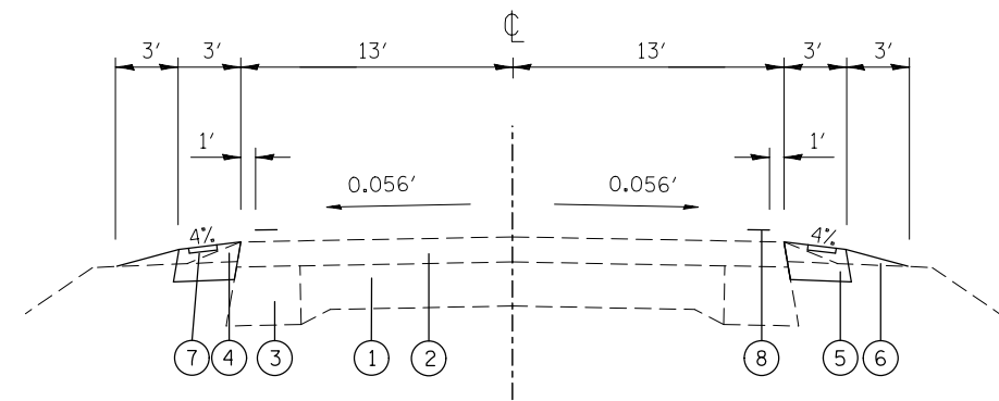
PROPOSED TYPICAL SECTION MILEPOINT 3.75 - 7.15
