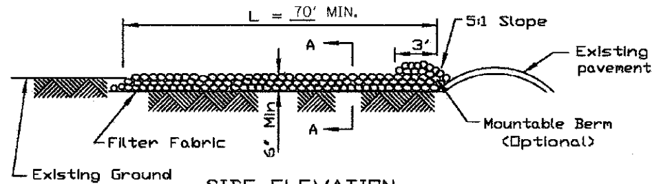
SIDE ELEVATION
