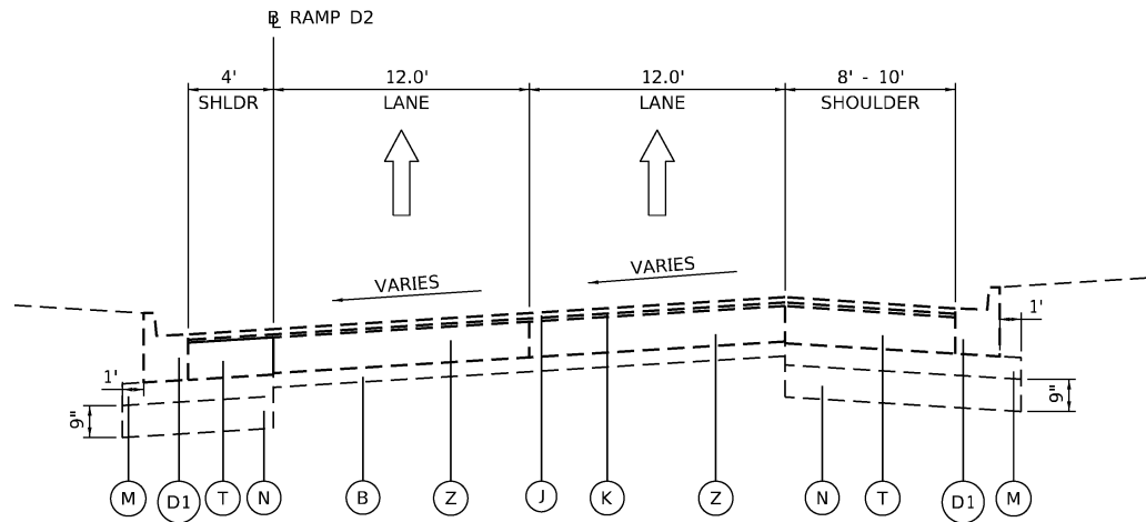
STONY ISLAND EXISTING RAMP D2
