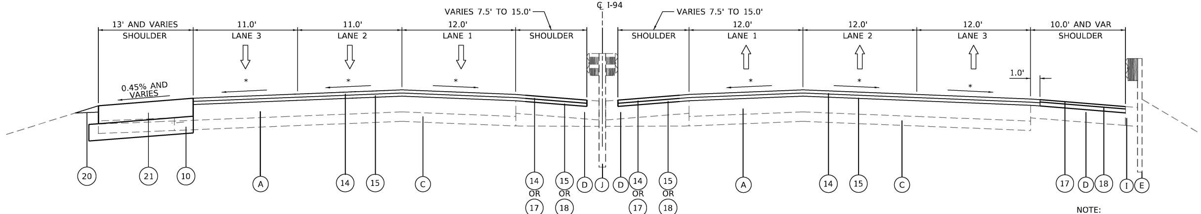
I-94 PROPOSED TYPICAL SECTION
