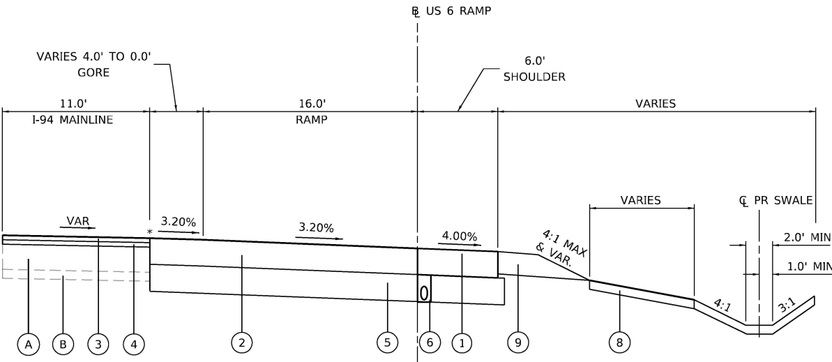
I-94 PROPOSED RAMP Y1 TYPICAL SECTION (LOOKING UPSTATION) STA 109+27.69 TO STA 111+26.69
