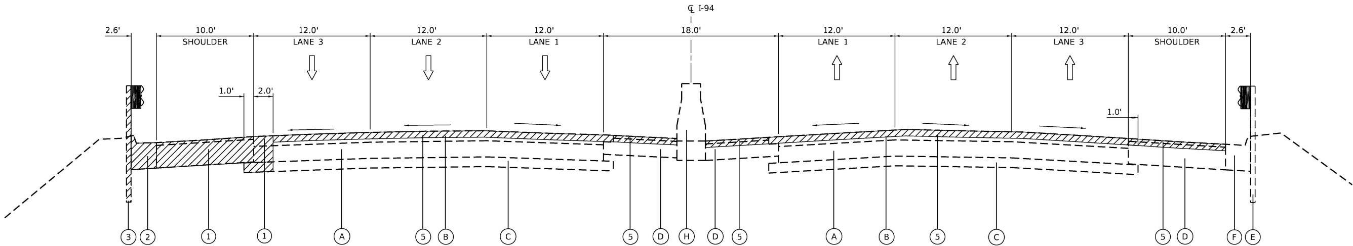
I-94 EXISTING TYPICAL SECTION LOOKING UPSTATION (EAST) STA 572+92.42 TO STA 579+78.80
