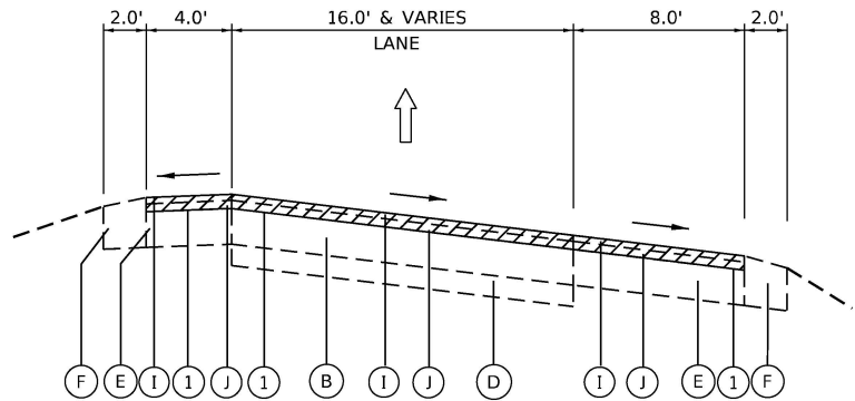
I-94 EXISTING RAMP TYPICAL SECTION
