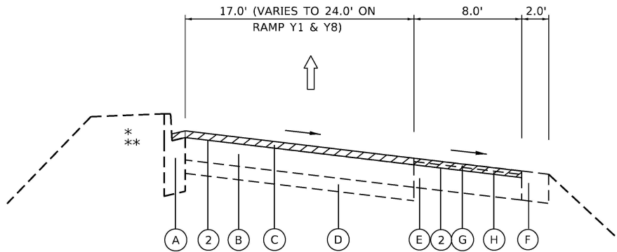
I-94 EXISTING RAMP TYPICAL SECTION
