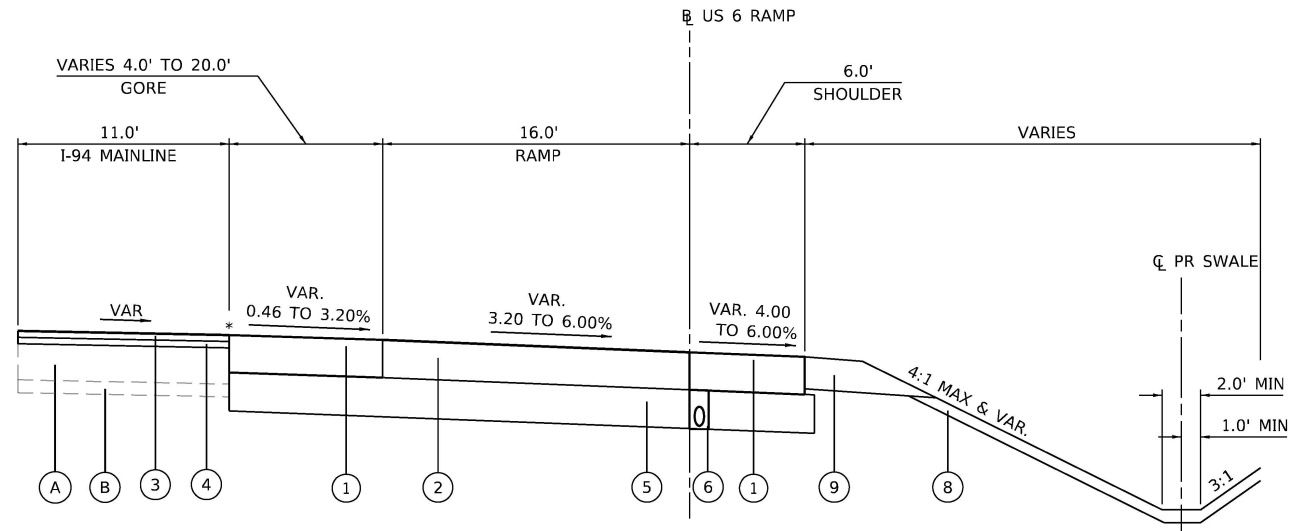
I-94 PROPOSED RAMP Y1 TYPICAL SECTION (LOOKING UPSTATION) STA 106+26.45 TO STA 109+27.69
