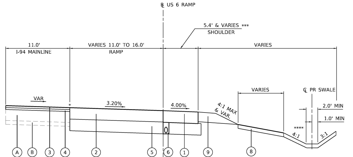
I-94 PROPOSED RAMP Y1 TYPICAL SECTION (LOOKING UPSTATION) STA 111+26.69 TO STA 113+65.40 (STA 113+65.40 RAMP ALIGNMENT = STA 583+77.84 MAINLINE ALIGNMENT)
