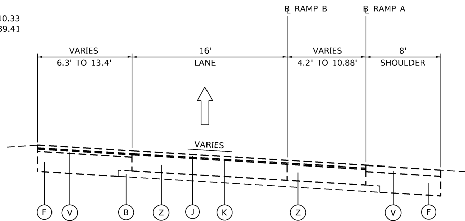
STONY ISLAND EXISTING RAMP A AND RAMP B (LOOKING UPSTATION) RAMP B STA 507+26.22 TO 509+32.20
