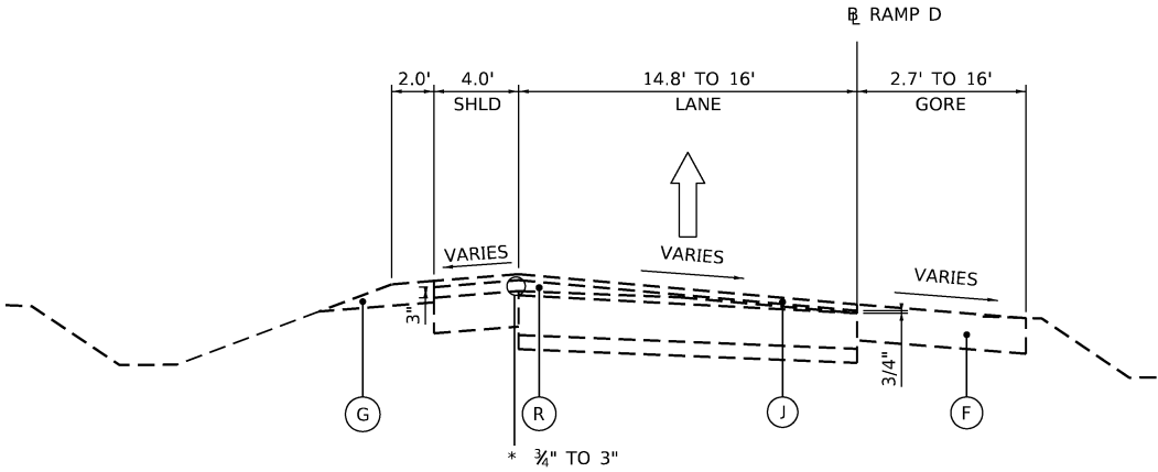
STONY ISLAND EXISTING RAMP D (LOOKING UPSTATION) STA 309+48.53 TO STA 311+65.33
