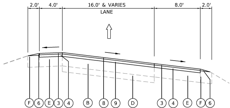
I-94 PROPOSED RAMP TYPICAL SECTION
