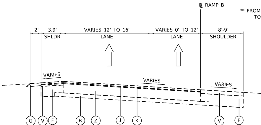
STONY ISLAND EXISTING RAMP B (LOOKING UPSTATION) STA 501+10.33 TO STA 505+33.35 e = |5.0% STA 501+26.70 TO STA 508+35.88
