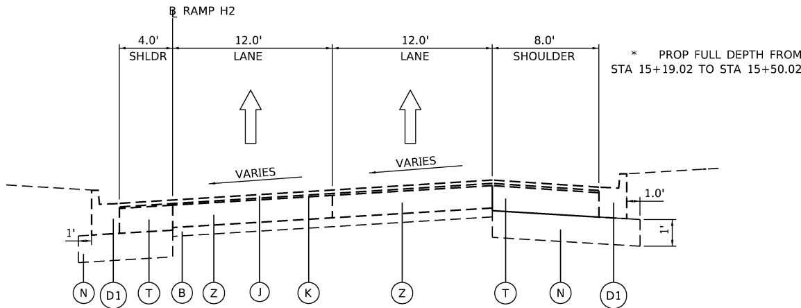
STONY ISLAND EXISTING RAMP H2
