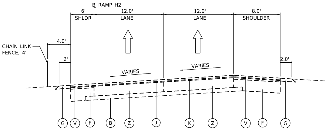
STONY ISLAND EXISTING RAMP H2
