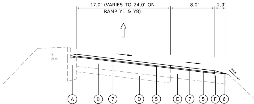
I-94 PROPOSED RAMP TYPICAL SECTION
