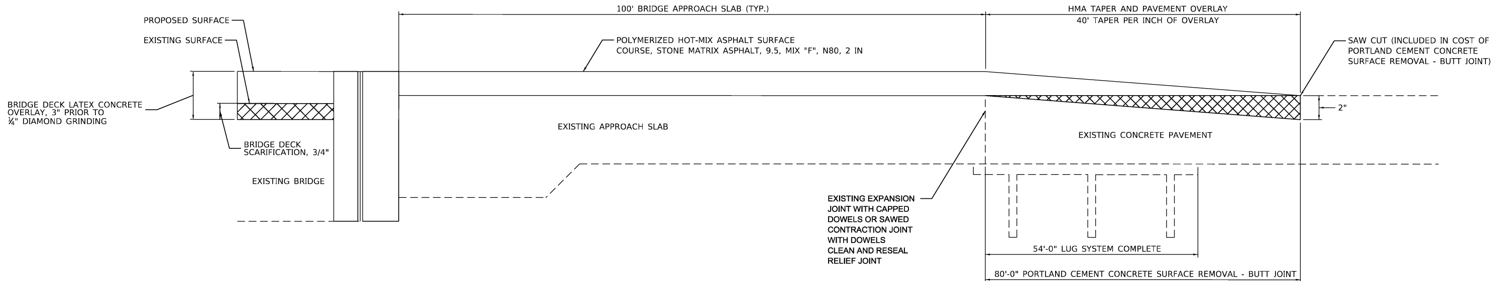
APPROACH PAVEMENT SMA OVERLAY DETAIL
