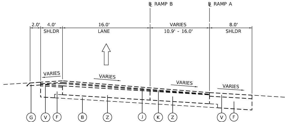
STONY ISLAND EXISTING RAMP A AND RAMP B (LOOKING UPSTATION) RAMP B STA 505+33.35 TO 507+26.22
