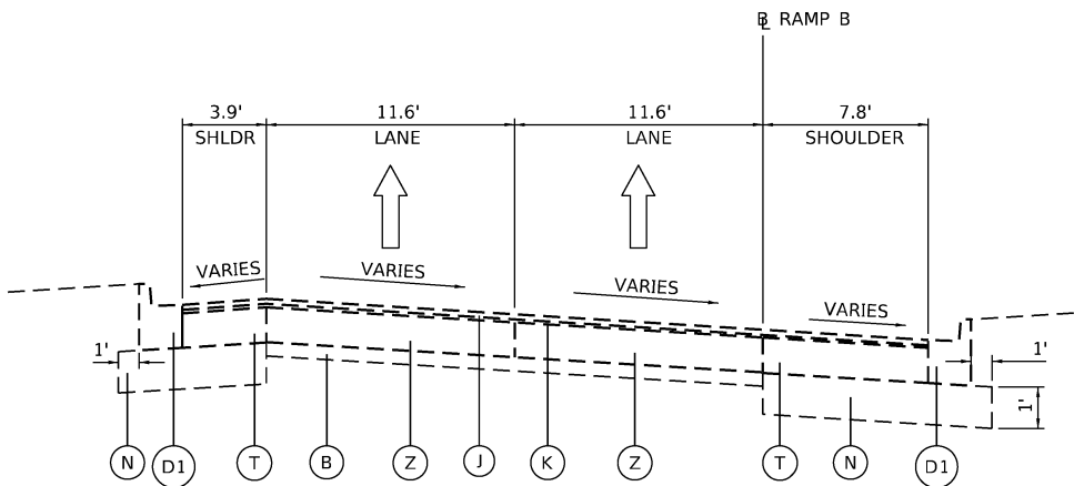
STONY ISLAND EXISTING RAMP B (LOOKING UPSTATION) STA 500+30.88 TO STA 500+79.13
