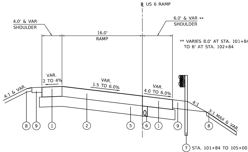
I-94 PROPOSED RAMP Y1 TYPICAL SECTION (LOOKING UPSTATION (NORTH)) STA 101+84.00 TO STA 106+26.45
