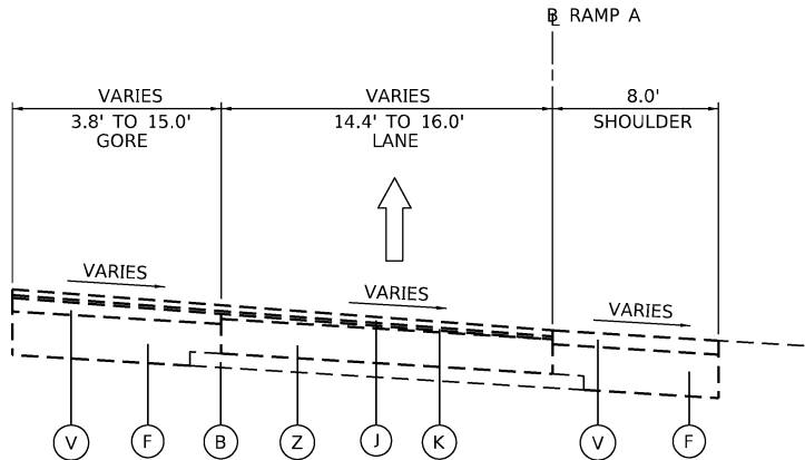
STONY ISLAND EXISTING RAMP A (LOOKING UPSTATION) STA 411+86.72 TO STA 412+74.93
