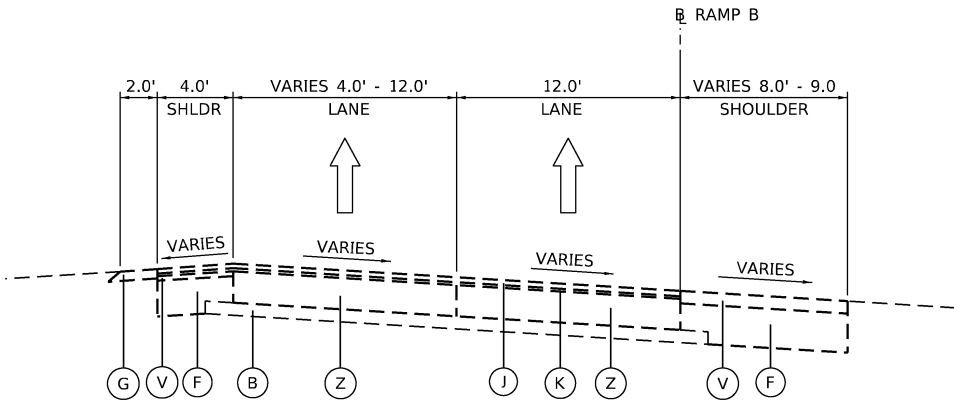
STONY ISLAND EXISTING RAMP B (LOOKING UPSTATION) STA 500+79.13 TO STA 501+10.33
