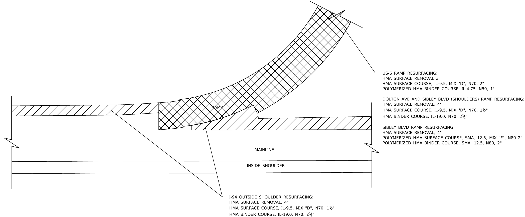
RAMP – GORE RESURFACING DETAIL
