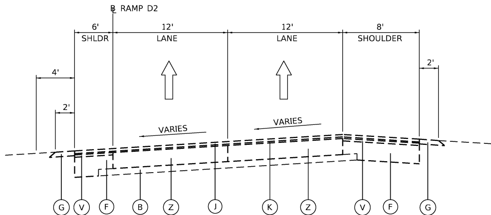
STONY ISLAND EXISTING RAMP D2
