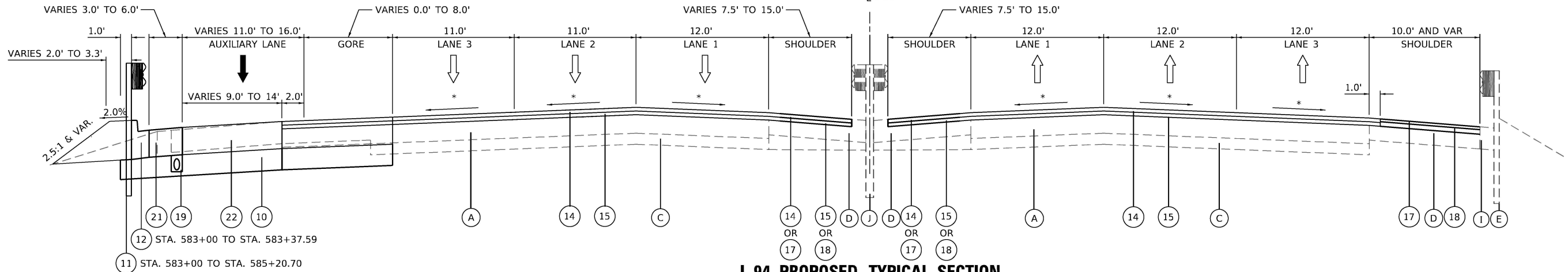
I-94 PROPOSED TYPICAL SECTION
