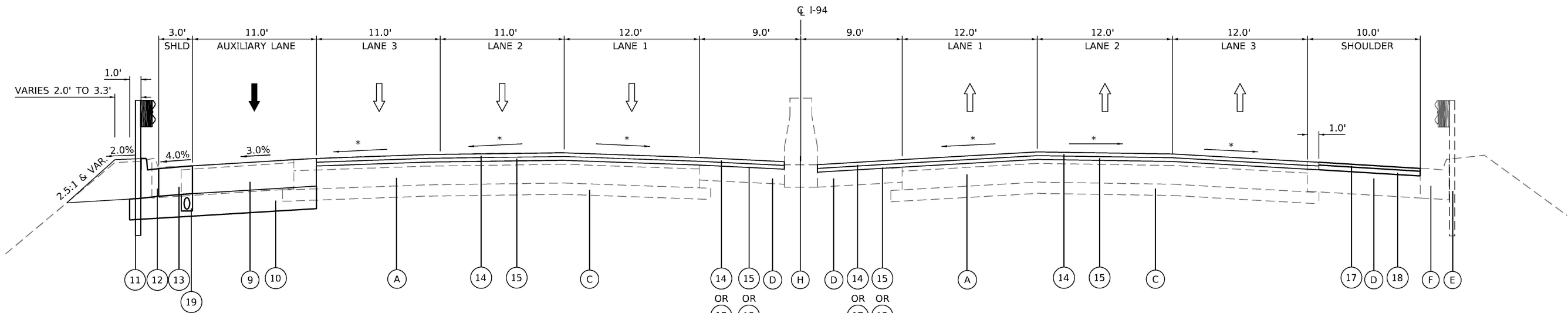
I-94 PROPOSED TYPICAL SECTION LOOKING UPSTATION (EAST) STA 572+92.42 TO STA 579+78.80
