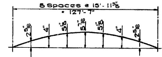
CAMBER DIAGRAM
