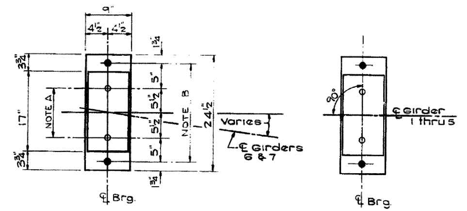
PLAN - ABUTMENTS
