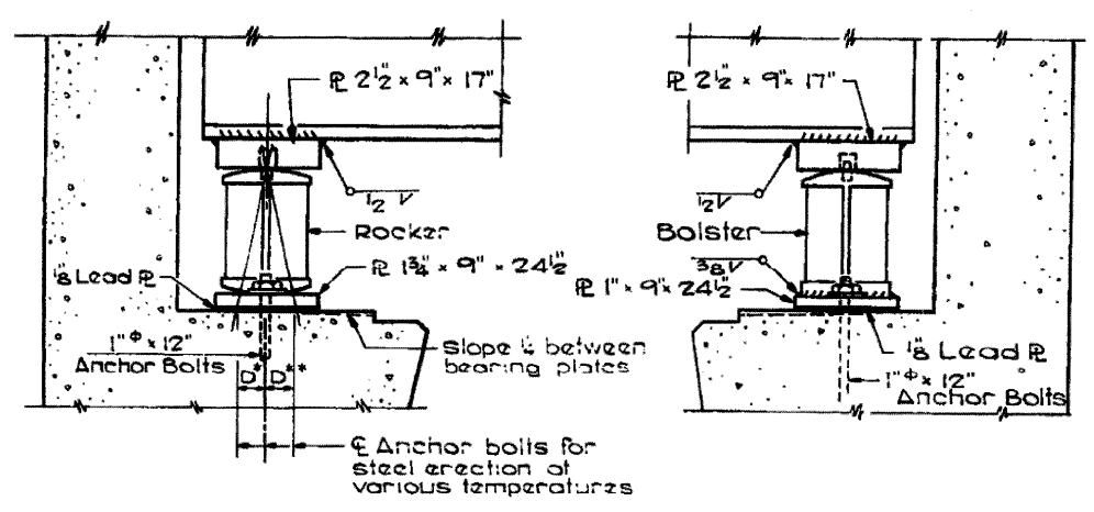
SOUTH ABUTMENT
