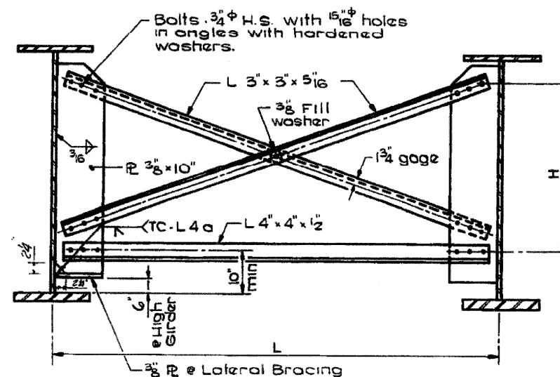
INTERMEDIATE CROSS-FRAMES
