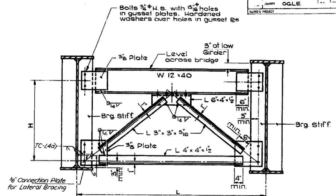
END CROSS-FRAMES
