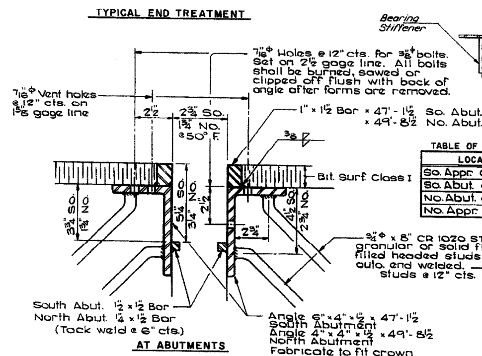
ARMOR ANGLE DETAILS
