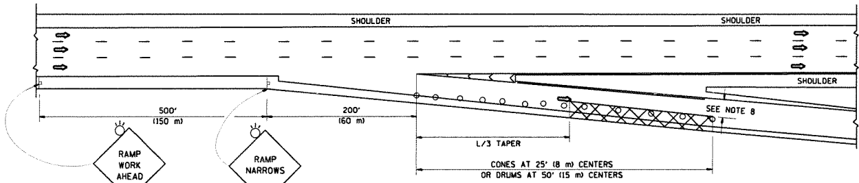
TYPICAL EXIT RAMP
