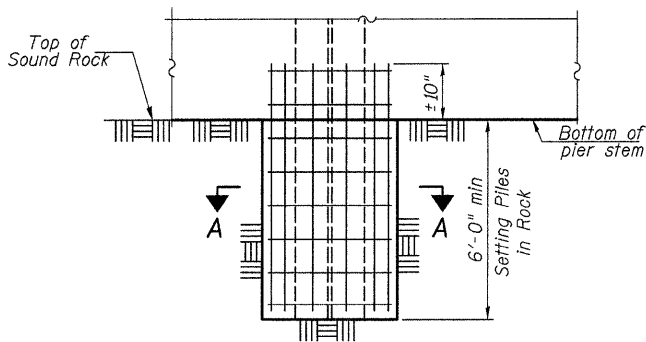
PIER ELEVATION
