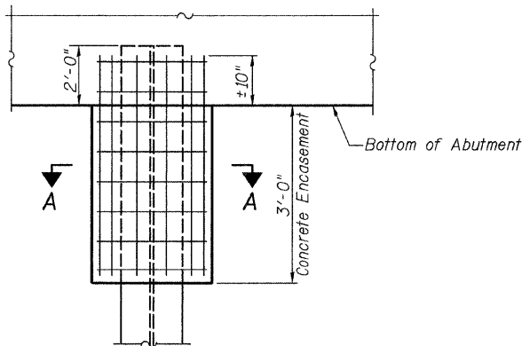
ABUTMENT ELEVATION
