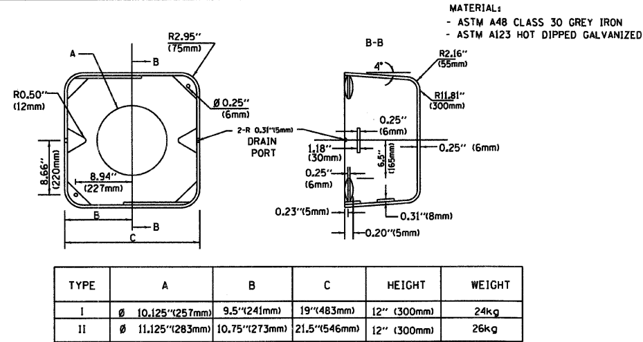
SHROUD DETAIL
