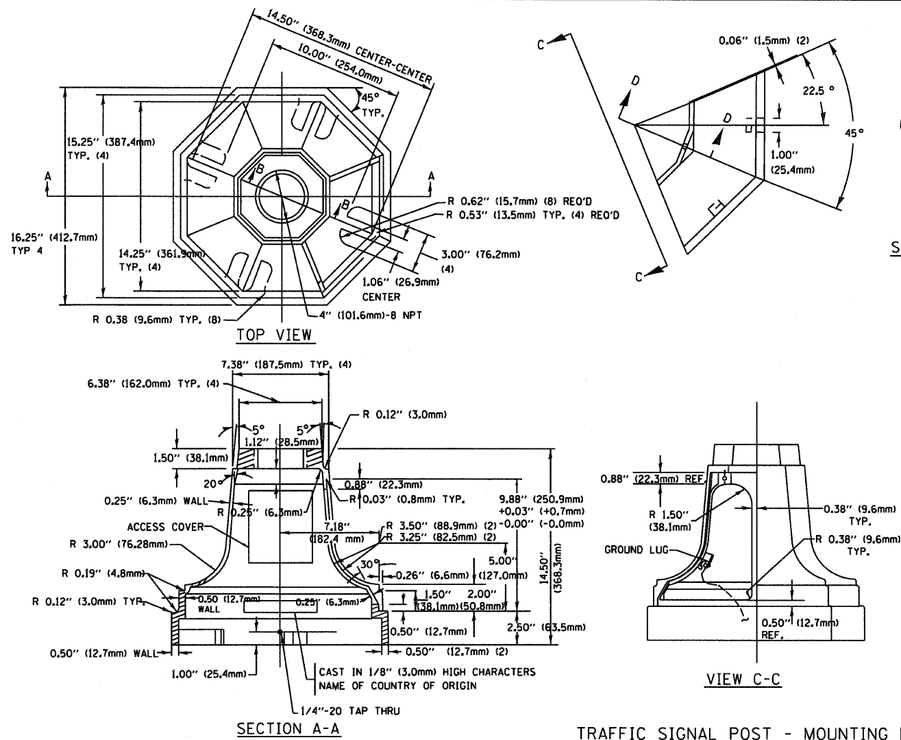
TRAFFIC SIGNAL POST - MOUNTING BASE - TYPE A
