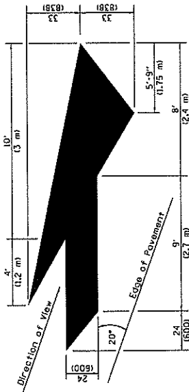
LANE-REDUCTION ARROW
