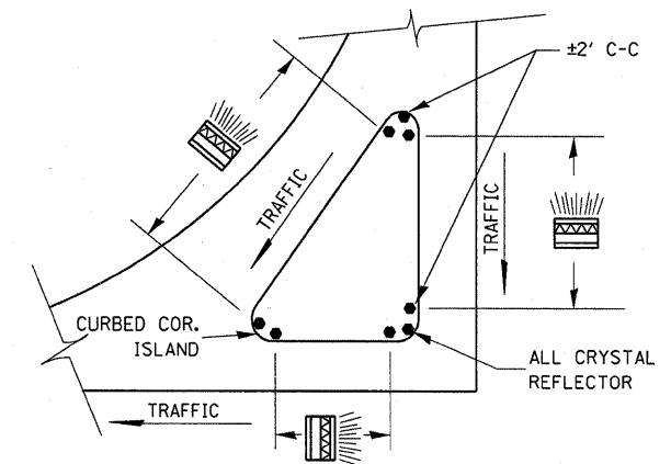
PRISMATIC REFLECTORS
