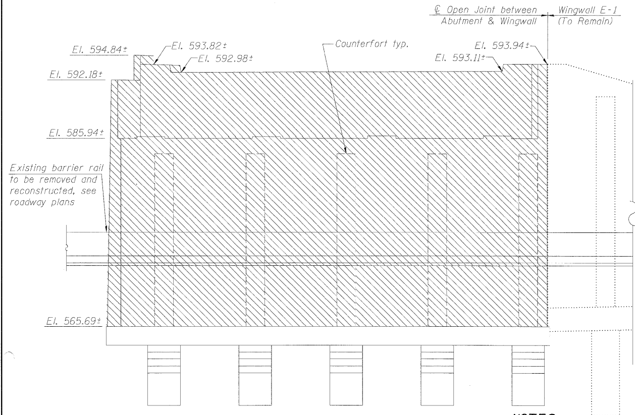
ELEVATION ABUTMENT C
