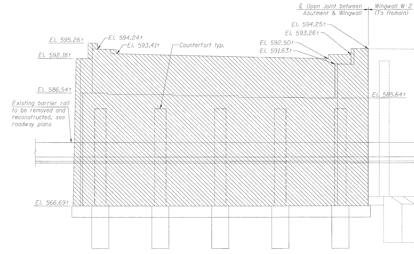
ELEVATION ABUTMENT D
