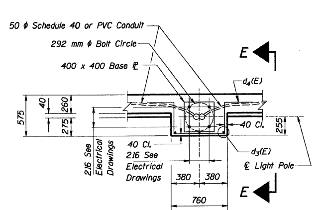
LIGHT POLE PLAN
